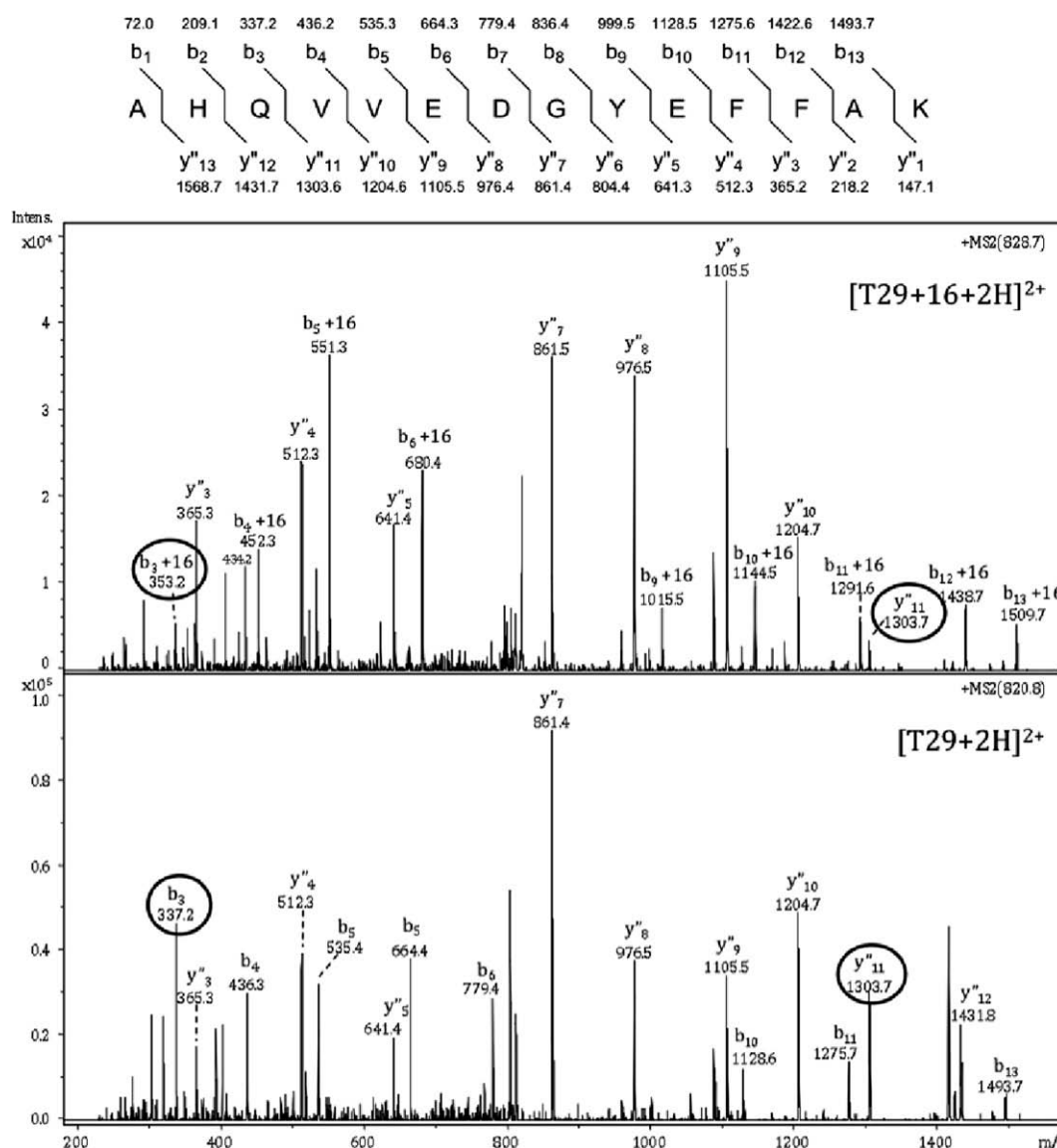
Figure 6. MS/MS spectra of peptide T29 and T29 + 16 Da. Peptide T29 + 16 Da shows a mass increase of 16 Da for fragment b_3 compared with peptide T29 . The spectrum of peptide T29 + 16 Da also shows y''_{11} , unchanged compared with peptide T29 , thus confirming that the oxidation has taken place at one of the following amino acid residues; Ala247, His248 or Gln249.
