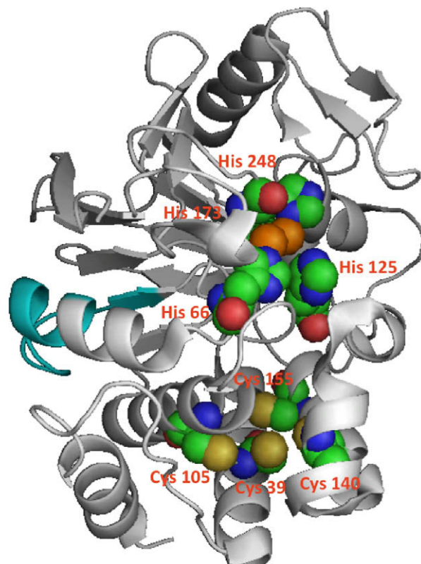
Figure 9. The X-ray structure of PP1 with the active site highlighted (His66, His125, His173, and His248), the new metal center highlighted (Cys39, Cys105, Cys140, and Cys155), and the potential oxidation sites on peptide T10 marked in light blue. The figure is based on the X-ray structure (3e7b) obtained from the protein data bank. 3b
