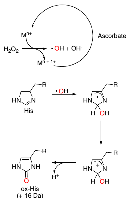
Figure 1. General outline of the Fenton/Fenton-like reaction (top) and an example of how the reactive oxygen species generated from that reaction oxidizes histidine.
