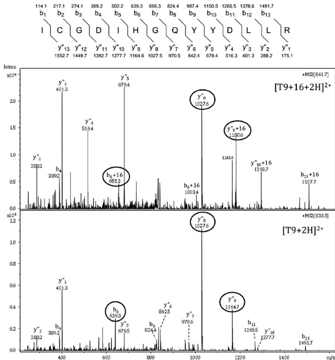
Figure 3. MS/MS spectra of peptides T9 and T9 + 16 Da. Peptide T9 + 16 Da shows a mass increase of 16 Da for fragments y_9' and y_{10}' compared with peptide T9 . The spectrum of peptide T9 + 16 Da also shows that fragment y_6' is unchanged compared with peptide T9 , thus confirming the oxidation of His66. The oxidation of His66 is also supported by a 16 Da increase in the mass of fragment b_6 in the spectrum of peptide T9 + 16 Da compared with peptide T9 .
