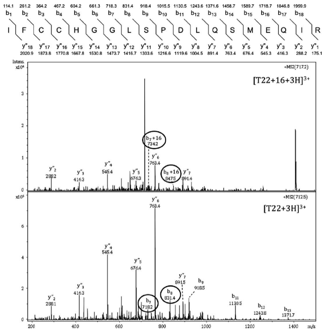
Figure 5. MS/MS spectra of peptides T22 and T22 + 16 Da . Peptide T22 + 16 Da shows a mass increase of 16 Da for fragments b_7 and b_8 compared with peptide T22 , thus indicating that the oxidation has taken place at one of the following amino acid residues; Ile169, Phe170, Cys171, Cys172, His173, Gly174 or Gly175.
