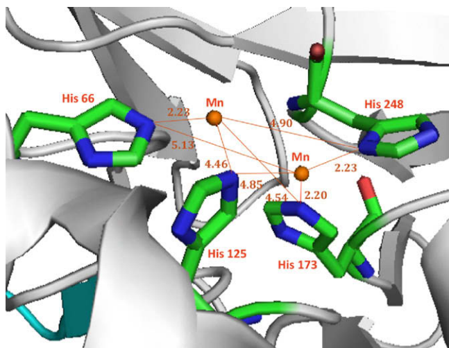
Figure 7. The active site of PP1 with the two metals marked in orange. The distance from the two metals to His is indicated in Å in the figure. The figure is based on the X-ray structure (3e7b) obtained from the protein data bank. 1
