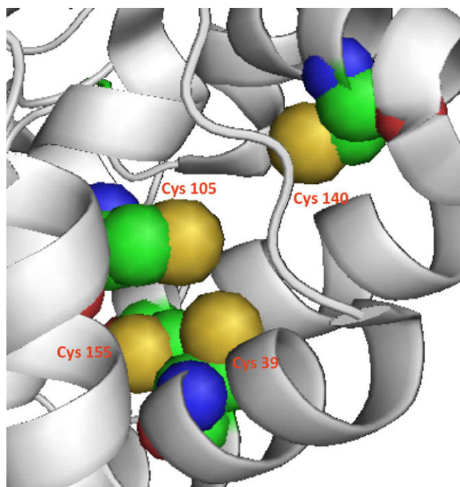
Figure 8. New metal center in PP1 \gamma formed upon addition of \text{Cu}^{2+} : Cys involved in \text{Cu}^{2+} coordination are highlighted (Cys39, Cys105, Cys140, and Cys155). The figure is based on the X-ray structure (3e7b) obtained from the protein data bank. 3b
