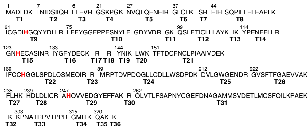
Figure 2. Peptide map for trypsin digested PP1 \gamma . His engaged in metal coordination is marked in red (peptide T9 , T15 , T22 , and T29 ).
